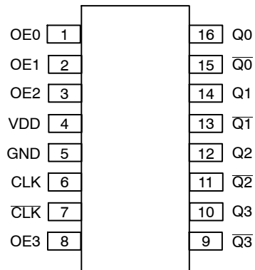
Figure 2. NB3L8504S Pinout, 16-pin TSSOP (Top View)
