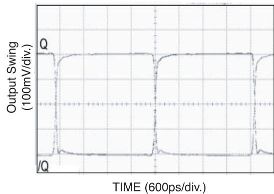
200MHz Clock
