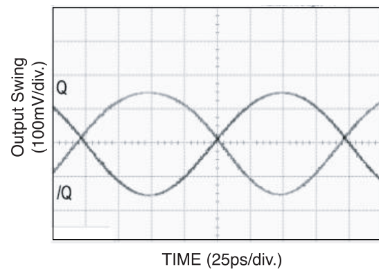
5GHz Clock
