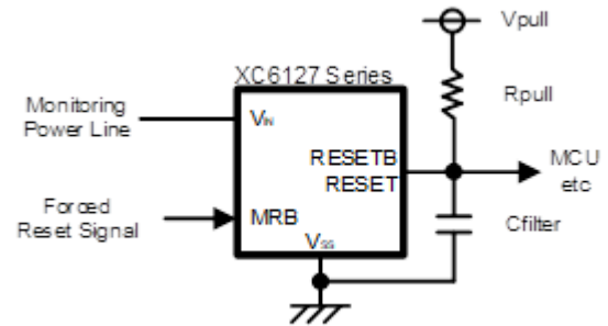
Counter measure circuit example (Nch-Open Drain Type)
