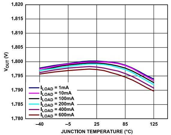
Figure 15. Output Voltage ( V_{OUT} ) vs. Junction Temperature ( T_J ) at Various Loads, V_{OUT} = 1.8 V
