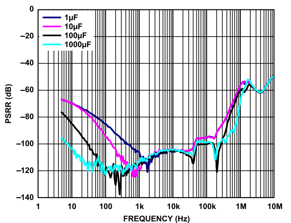
Figure 27. Power Supply Rejection Ratio (PSRR) vs. Frequency, Different C_{BYP} , V_{OUT} = 3.3\text{ V} , 400 mA Load, 500 mV Headroom
