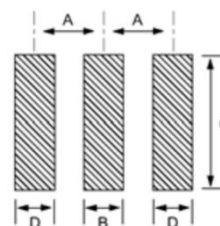
Figure 2) Land Pattern
