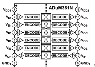
Figure 2. ADuM361N Functional Block Diagram
