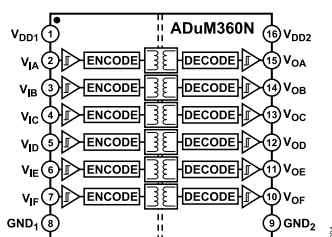
Figure 1. ADuM360N Functional Block Diagram
