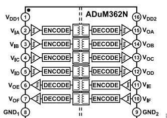
Figure 3. ADuM362N Functional Block Diagram
