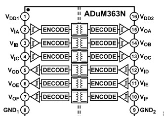
Figure 4. ADuM363N Functional Block Diagram
