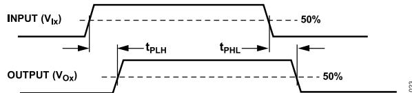
Figure 26. Propagation Delay Parameters
