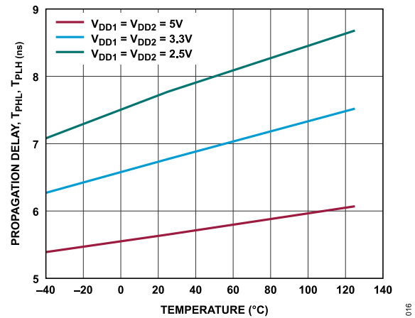
Figure 19. Propagation Delay, t_{PLH} , t_{PHL} vs. Temperature at Various Voltages
