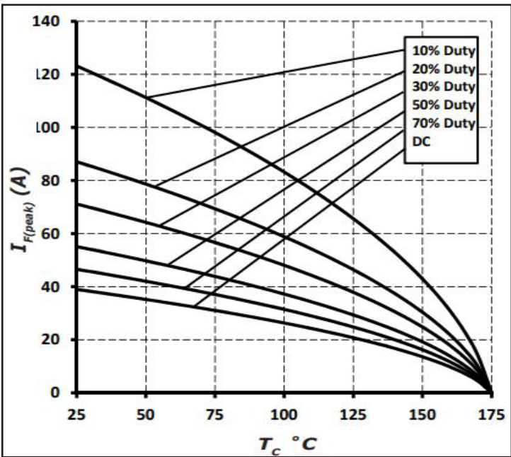
Figure 3 Current Derating
