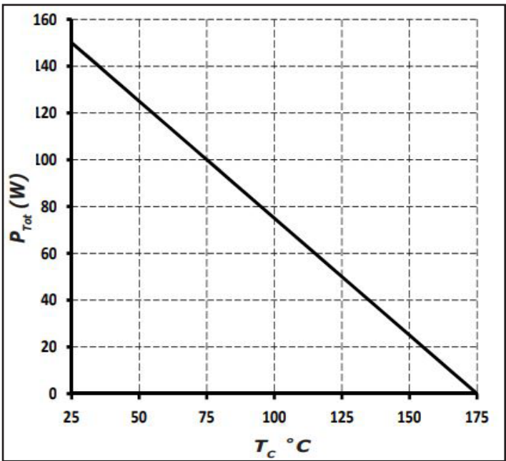
Figure 4 Power Derating
