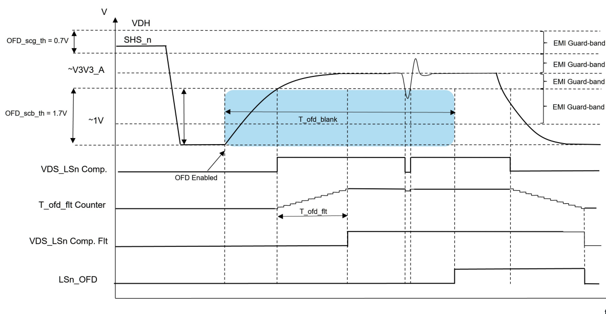
Figure 68. OFD Masking and deglitch filtering - LSn_OFD Example
