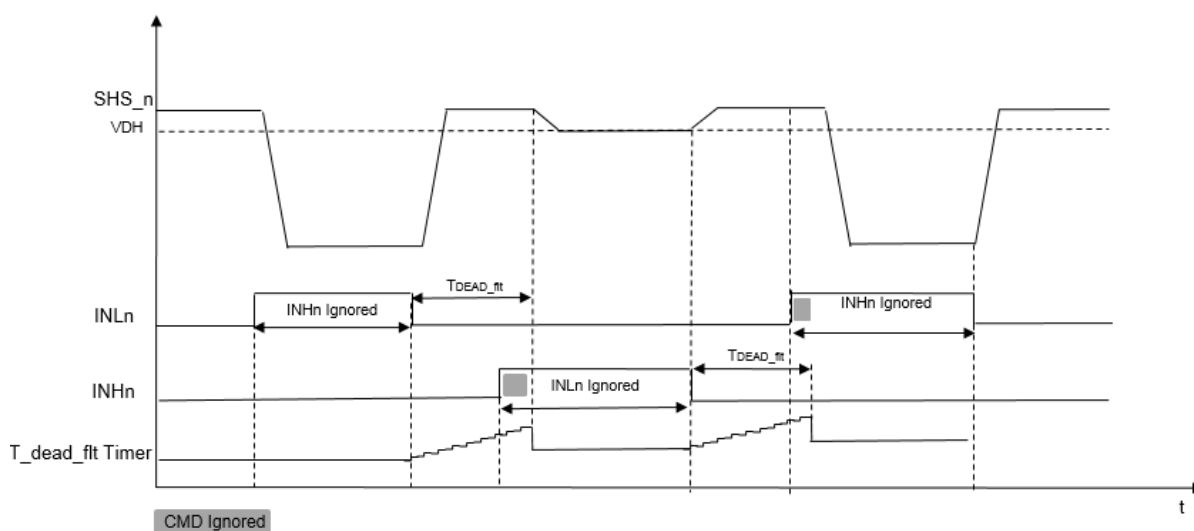
Figure 40. Dead Time Protection functional operation
