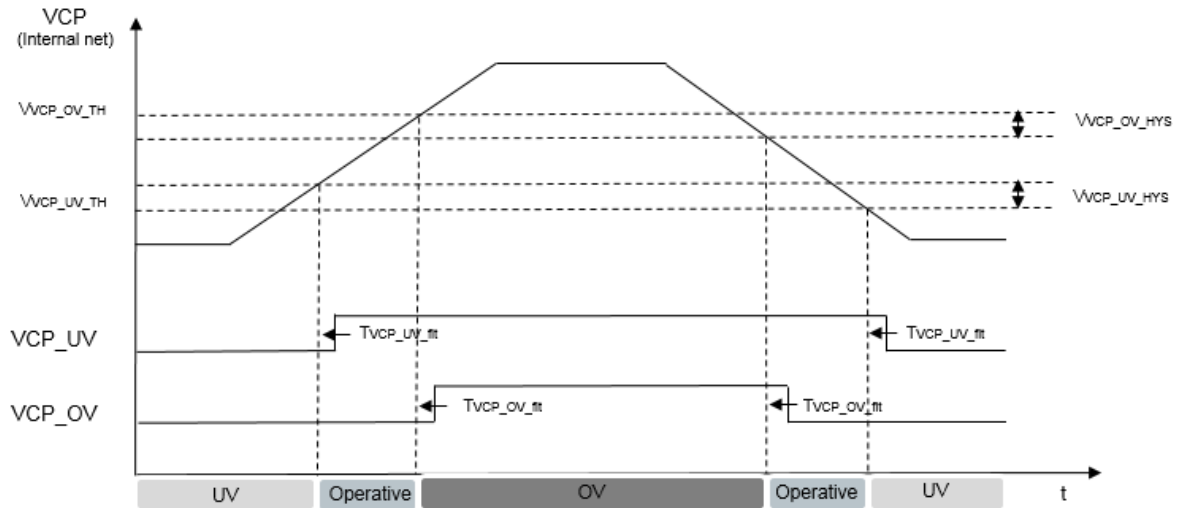
Figure 32. VCP operative range
