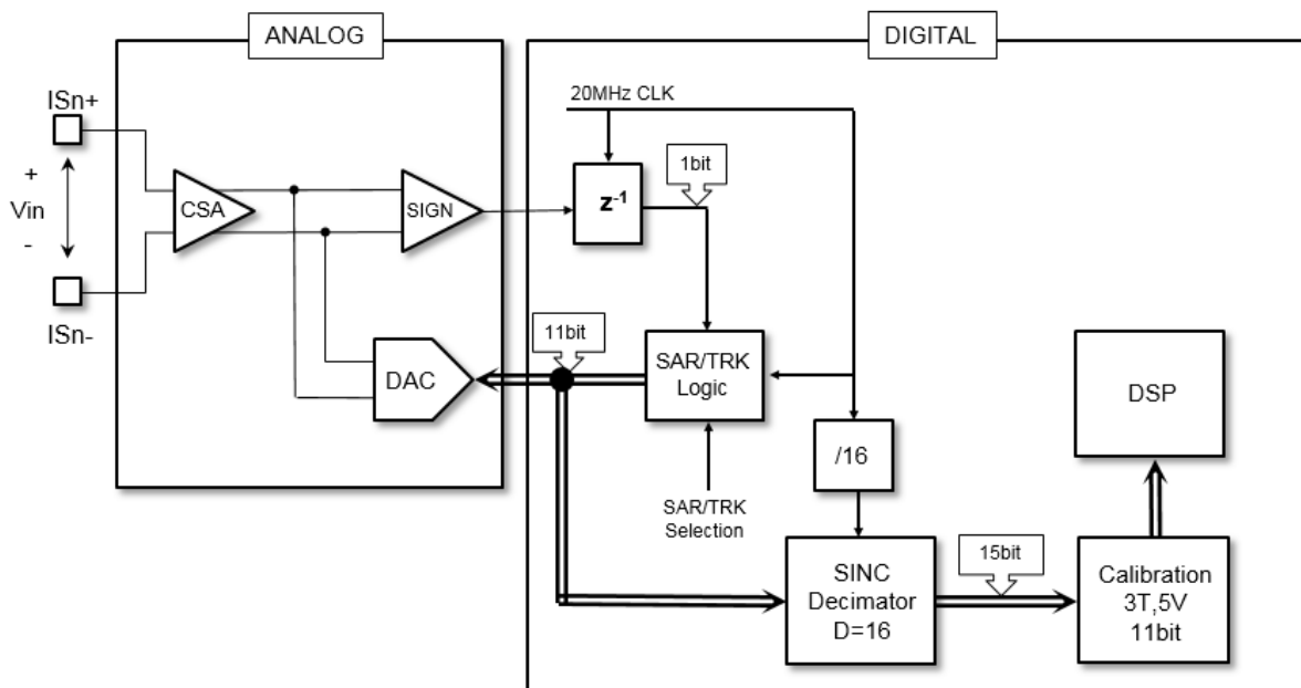
Figure 46. A/D Conversion simplified block diagram
