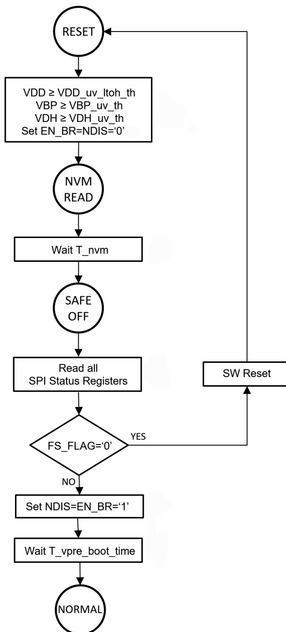
Figure 23. Power-Up diagram
