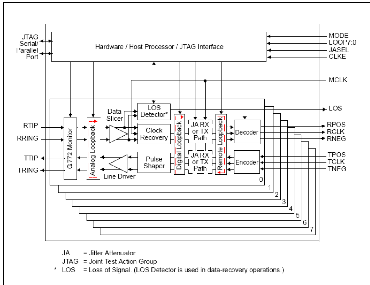
Figure 1 LXT384 Transceiver High-Level Block Diagram
