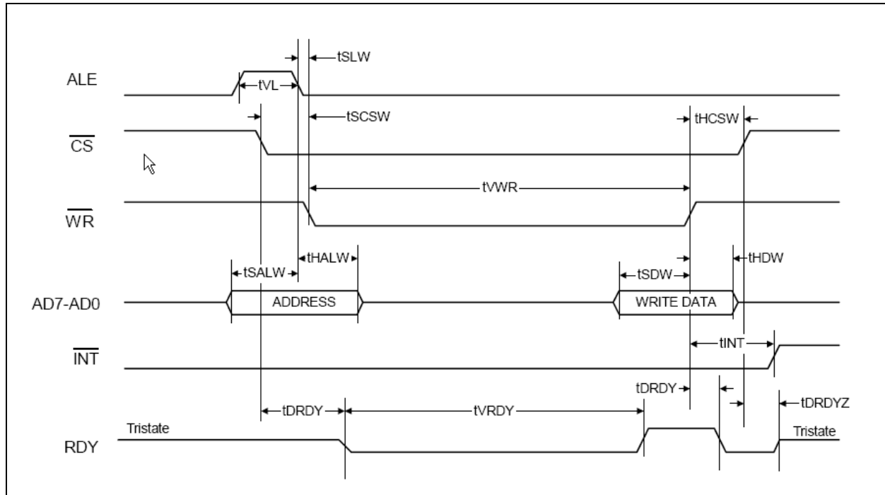
Figure 24 Intel® Processor Multiplexed Interface - Write Timing
