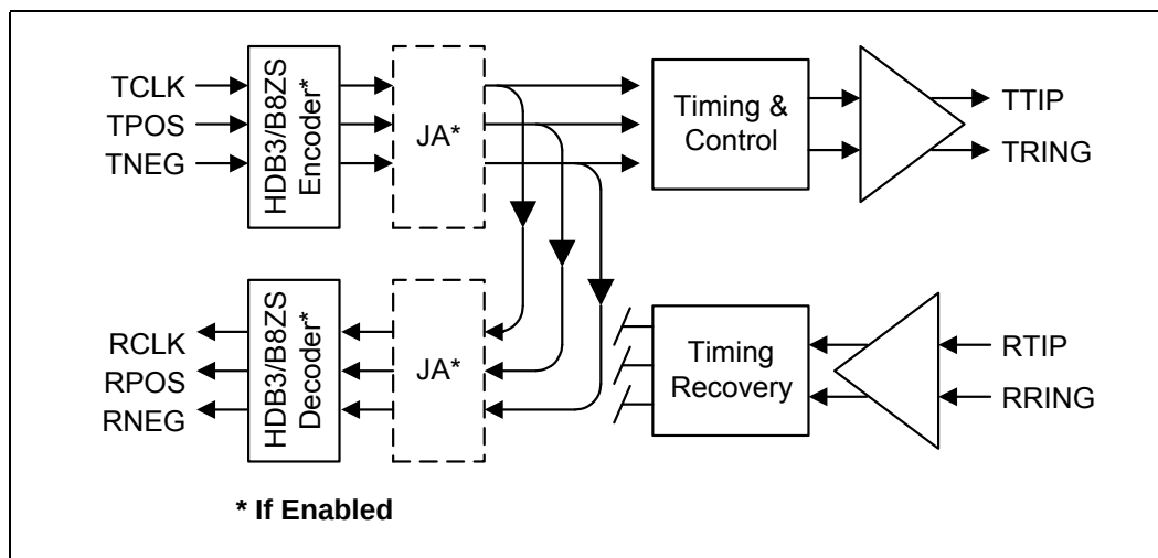
Figure 9 LXT384 Transceiver Digital Loopback
