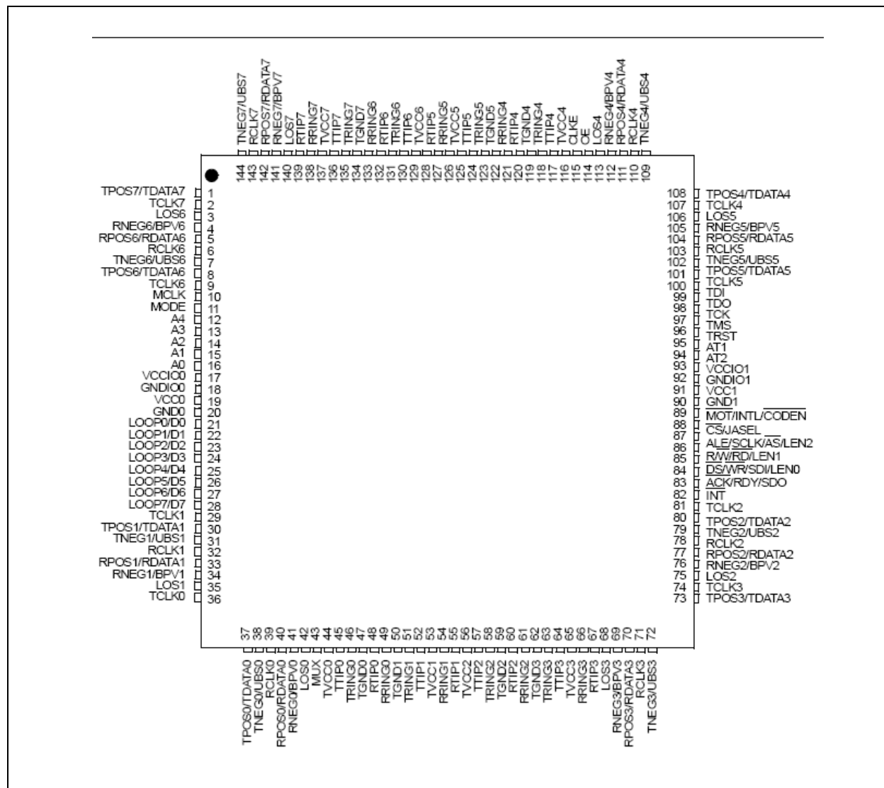
Figure 3 LXT384 Transceiver 144-Pin Assignments
