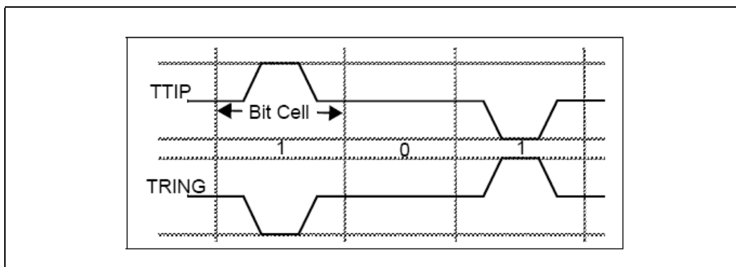
Figure 5 50 % AMI Encoding
