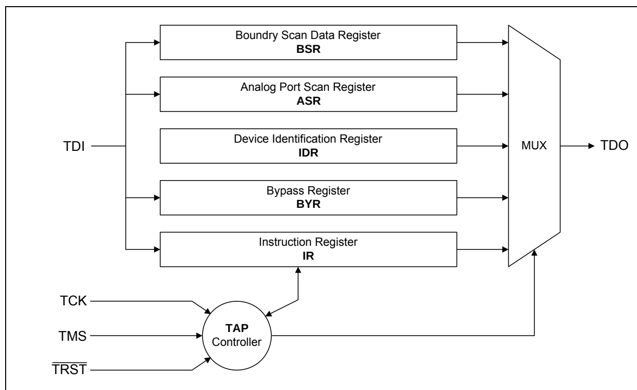
Figure 15 JTAG Architecture
