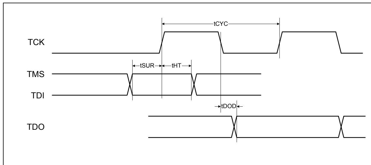
Figure 18 JTAG Timing
