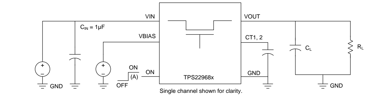
TEST CIRCUIT
