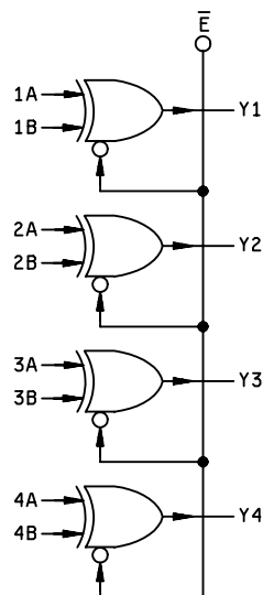
FIGURE 3. Logic diagram.
