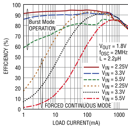
2A Buck Efficiency vs I LOAD , V OUT = 1.8V
