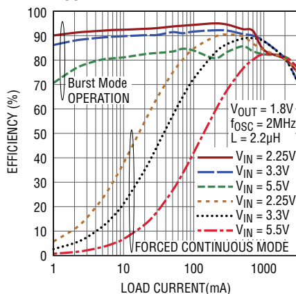
3A Buck Efficiency vs I LOAD , V OUT = 1.8V
