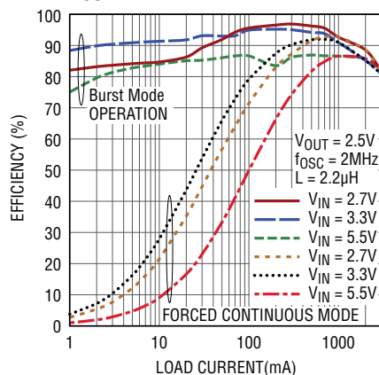
3A Buck Efficiency vs I LOAD , V OUT = 2.5V
