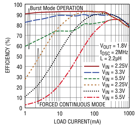
1A Buck Efficiency vs I LOAD , V OUT = 1.8V
