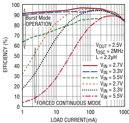
1A Buck Efficiency vs I LOAD , V OUT = 2.5V
