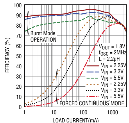
4A Buck Efficiency vs I LOAD , V OUT = 1.8V
