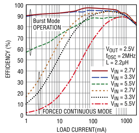
2A Buck Efficiency vs I LOAD , V OUT = 2.5V
