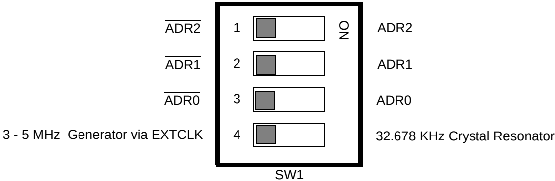
FIGURE 1-4 Configuration Dip-Switch - SW1
