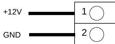
FIGURE 2-6 P12: +12V Power Connector
