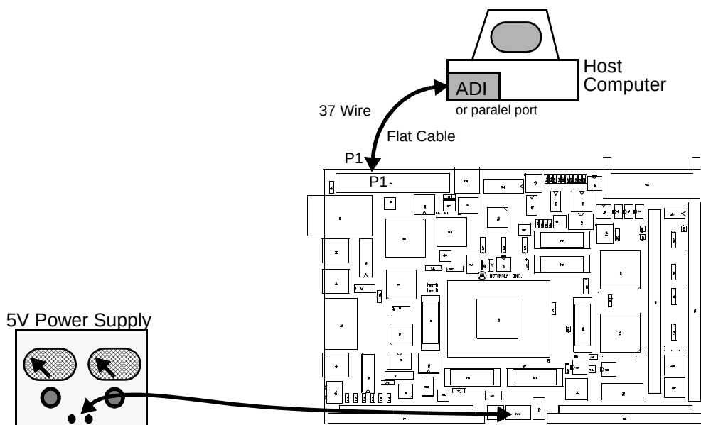
FIGURE 2-3 Host Controlled Operation Scheme
