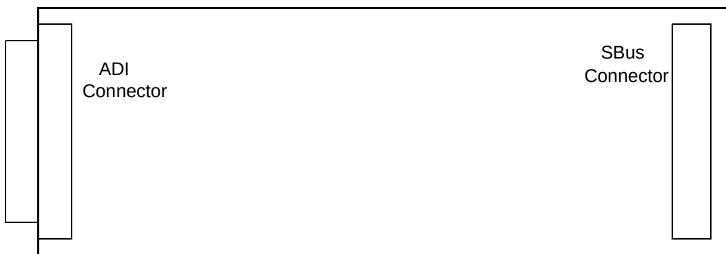
FIGURE B-3 ADI board for SBus
