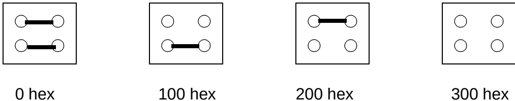
FIGURE B-2 JG1 Configuration Options
