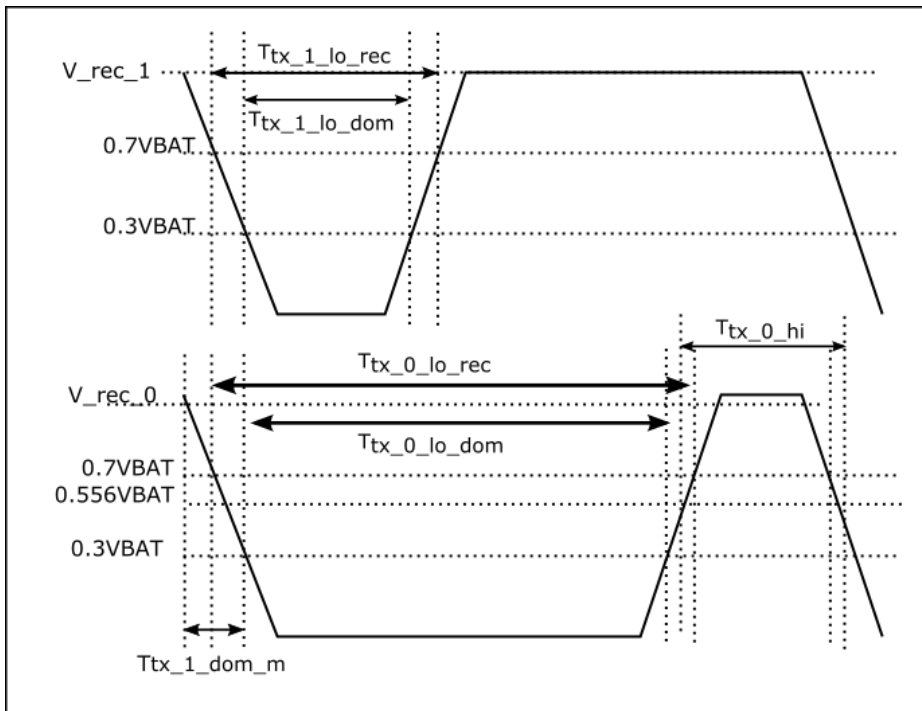
Figure 8-7. Logic Low and High CXPI BUS Waveform
