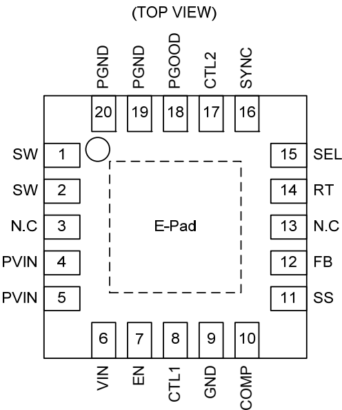
VQFN20SV4040
