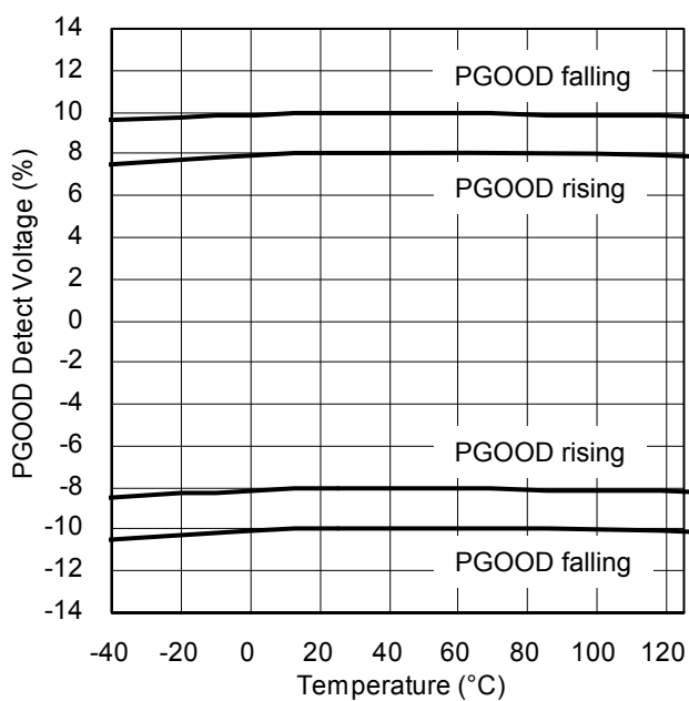
Figure 16. PGOOD DETECT Voltage vs Temperature
