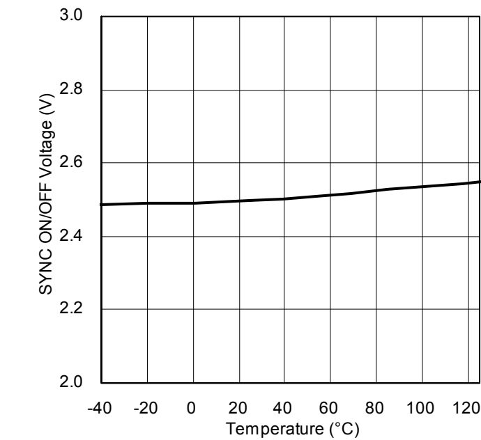
Figure 15. SYNC ON/OFF Voltage vs Temperature
