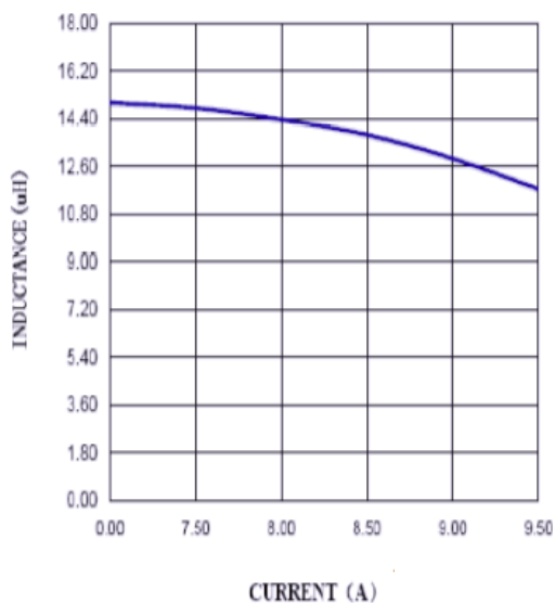
ASPI-1306T-150M
