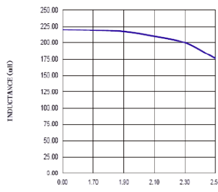
ASPI-1306T-221M
