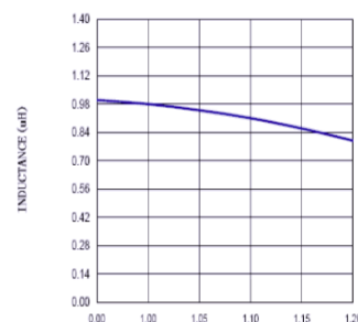
ASPI-1306T-102M
