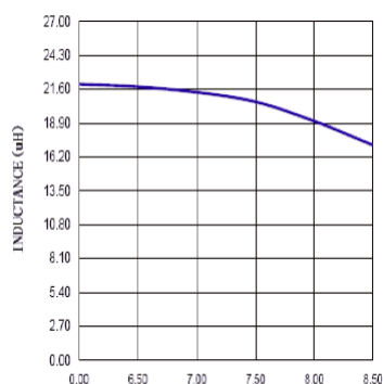
ASPI-1306T-220M
