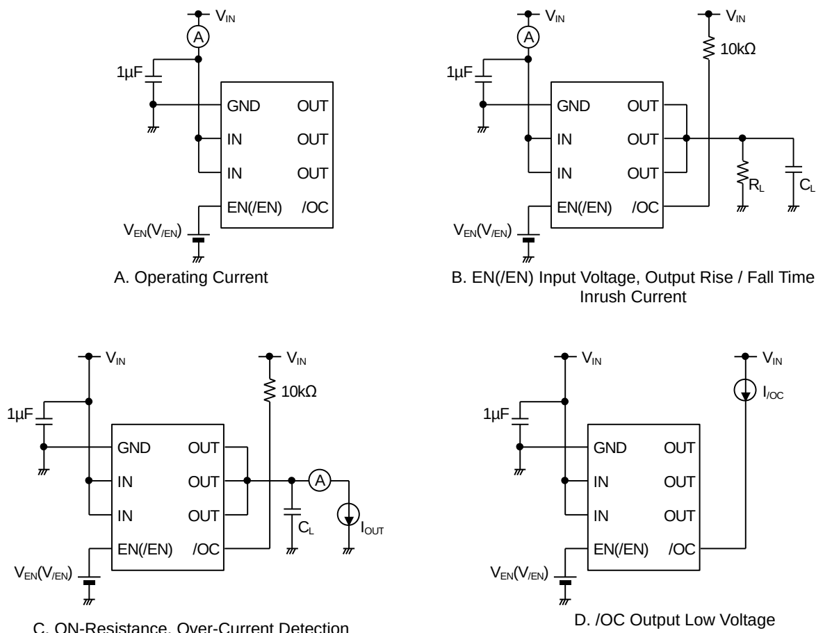
Figure 1. Measurement Circuit
