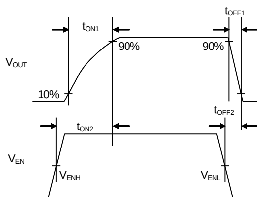
Figure 2. Timing Diagram (BD82006FVJ-M)
