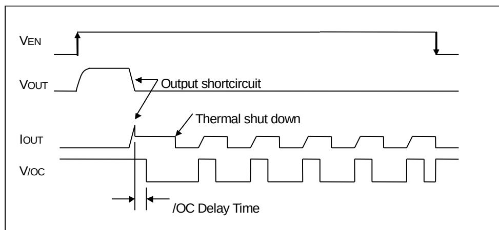
Figure 40. Over-Current Detection, Thermal Shutdown Timing (BD82006FVJ-M)
