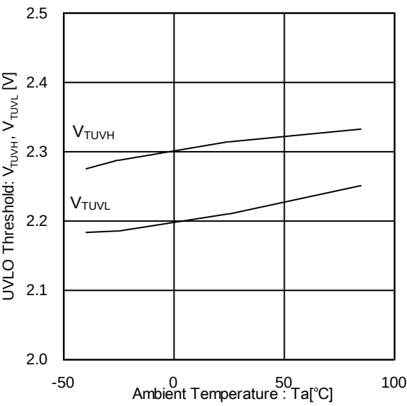
Figure 18. UVLO Threshold Voltage vs Ambient Temperature
