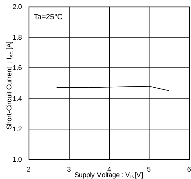
Figure 14. Short Circuit Current vs Supply Voltage
