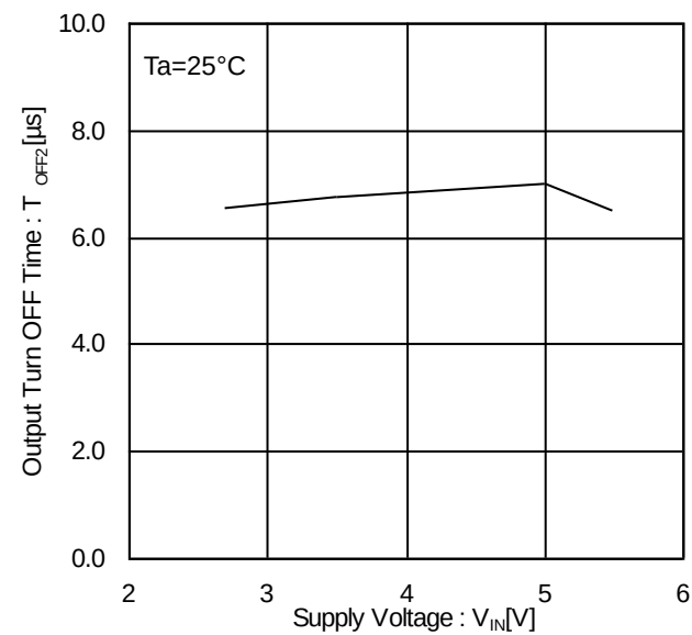
Figure 26. Output Turn OFF Time vs Supply Voltage
