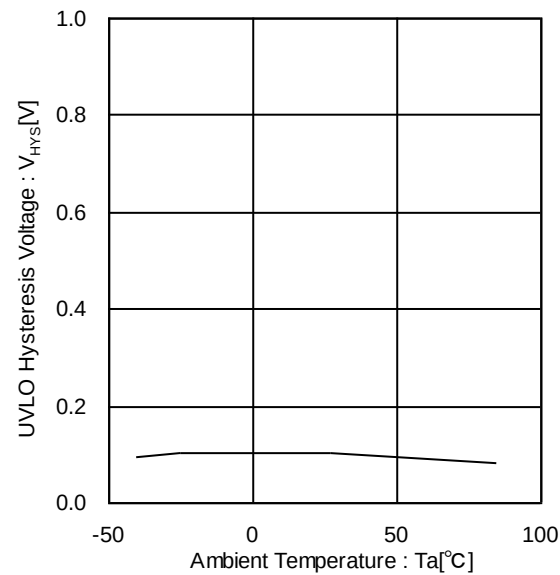
Figure 19. UVLO Hysteresis Voltage vs Ambient Temperature
