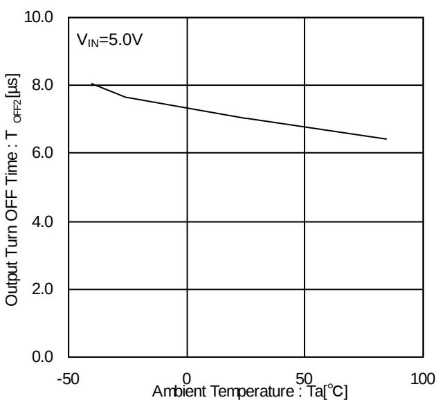
Figure 27. Output Turn OFF Time vs Ambient Temperature
