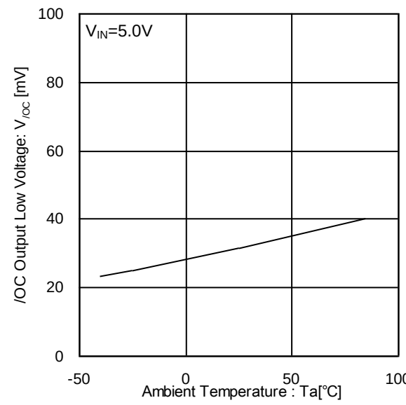
Figure 17. /OC Output Low Voltage vs Ambient Temperature
