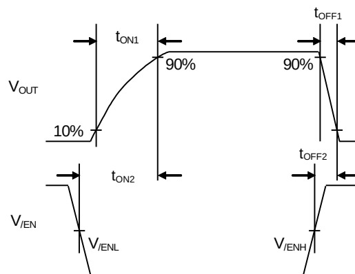
Figure 3. Timing Diagram (BD82007FVJ-M)
