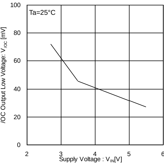
Figure 16. /OC Output Low Voltage vs Supply Voltage
