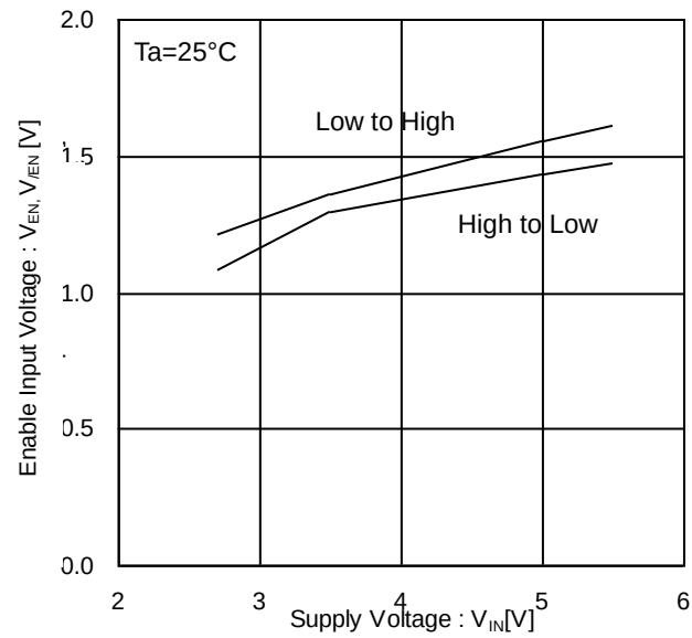
Figure 8. EN, /EN Input Voltage vs Supply Voltage
