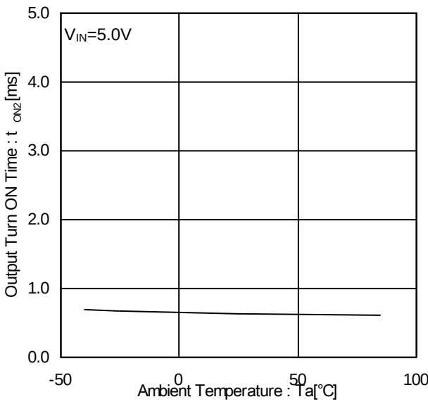
Figure 23. Output Turn ON Time vs Ambient Temperature
