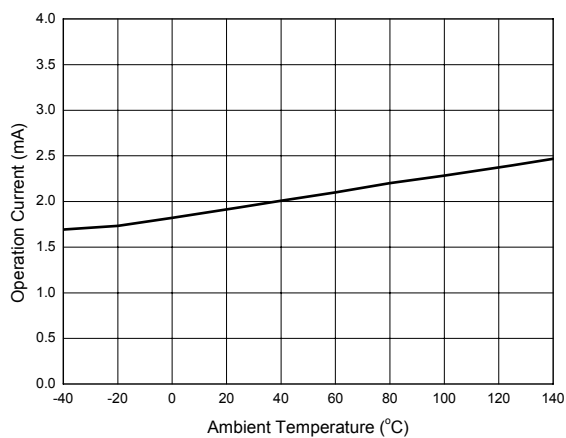
Figure 7. Operation Current vs. Ambient Temperature
