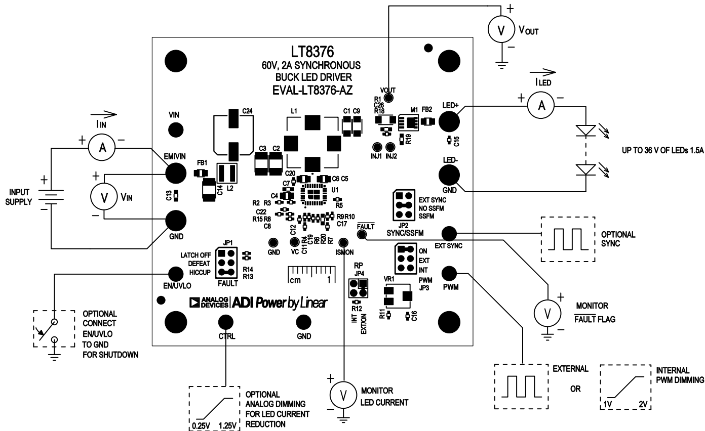
Figure 1. Setup Drawing for EVAL-LT8376-AZ
