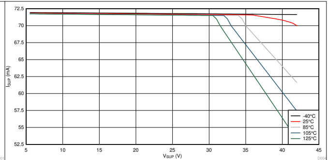
Figure 7-2. I_{SUP} vs V_{SUP} Across Temperature
