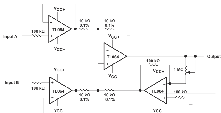
Figure 9-3. Instrumentation Amplifier
