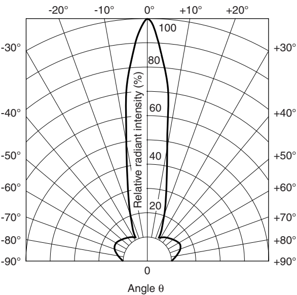
Fig. 2 Radiation Diagram
