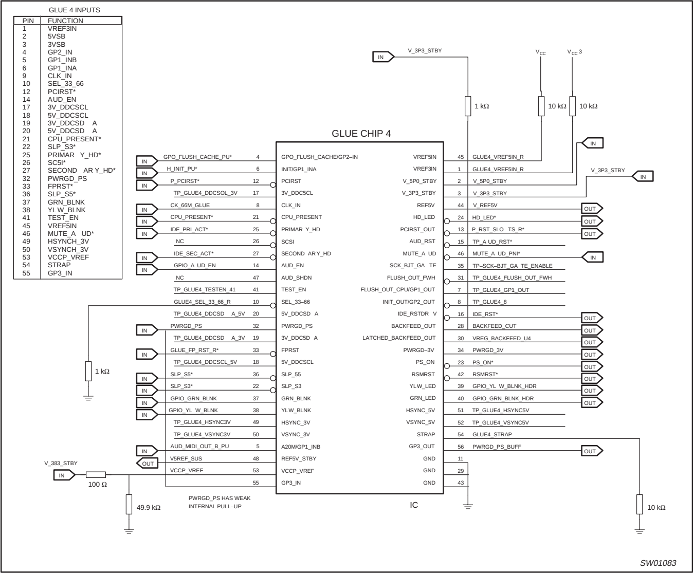
Figure 1. Typical application
