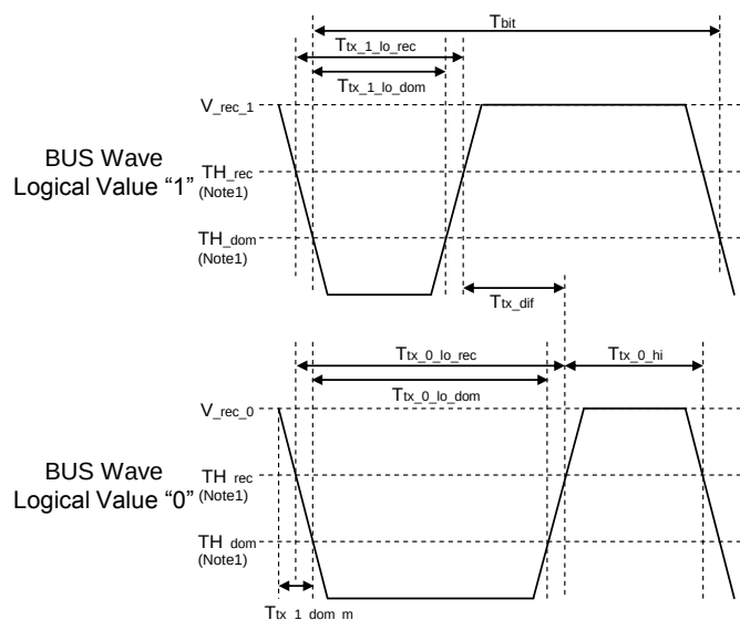
Figure 18. BUS Waves of Logical Value 1, 0
