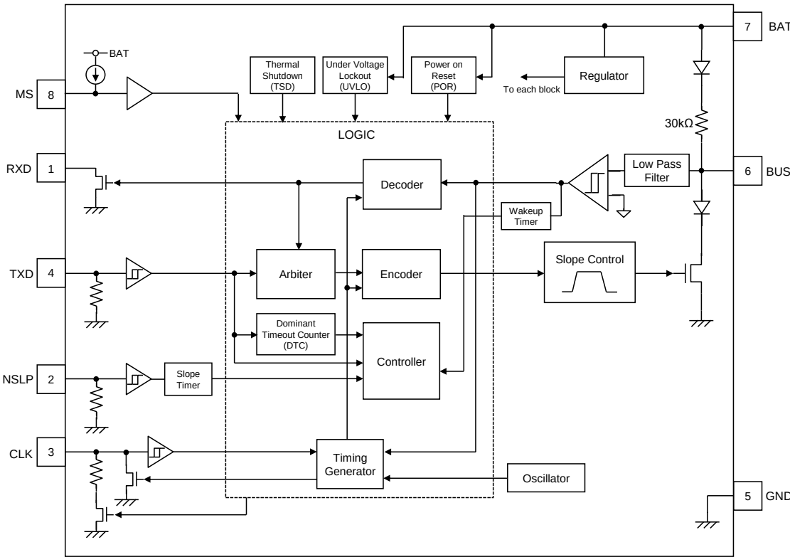
Figure 3. Block Diagram
