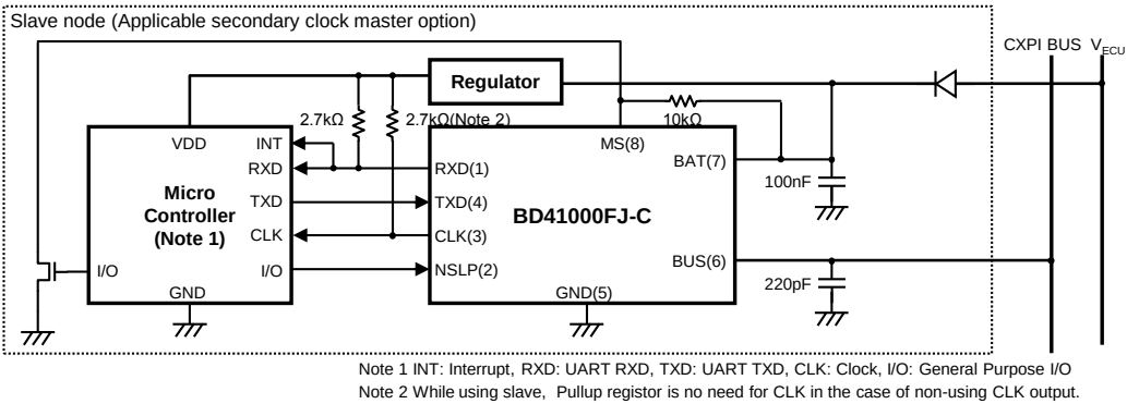
Figure 19. Application Example of Secondary Clock Master Option
