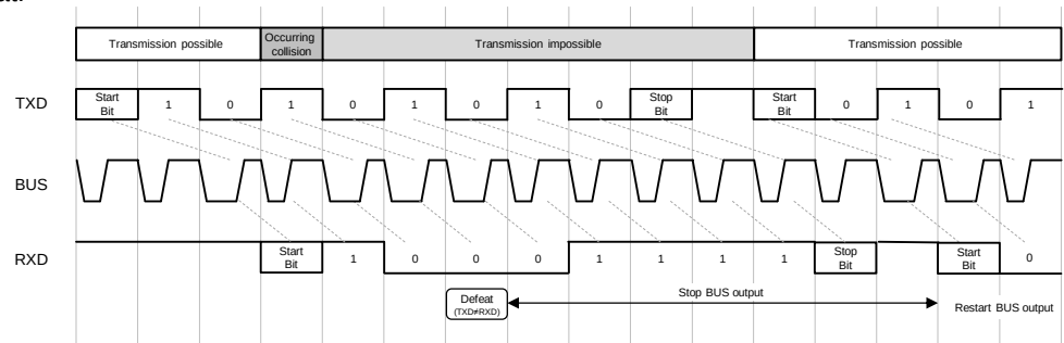
Figure 16. Arbitration Function (When the Collision is detected after Data Transmission)
