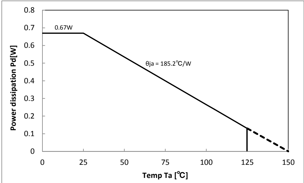
Figure 20. Power Dissipation
