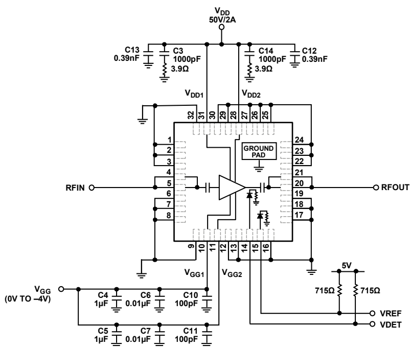
Figure 50. Basic Connection
