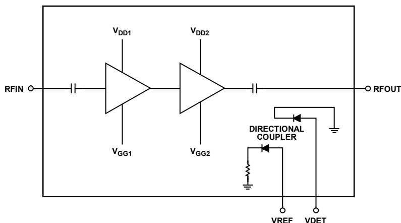
Figure 49. Basic Block Diagram
