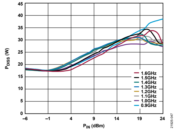
Figure 47. P_{DISS} vs. P_{IN} , Drain Bias Pulse Width = 50 \mu s at 5% Duty Cycle, T_{BASE} = 85^{\circ}\text{C}
