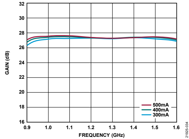
Figure 34. Gain vs. Frequency at Various I_{DQ} Currents, P_{IN} = 19 dBm
