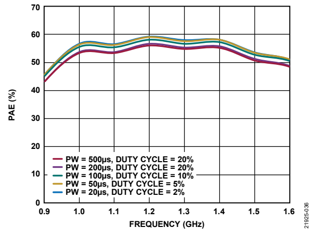
Figure 36. PAE vs. Frequency at Various Pulse Widths and Duty Cycles, P_{IN} = 16 dBm
