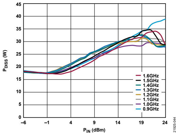
Figure 44. P_{DISS} vs. P_{IN} , Drain Bias Pulse Width = 20 \mu s at 2% Duty Cycle, T_{BASE} = 85^{\circ}\text{C}
