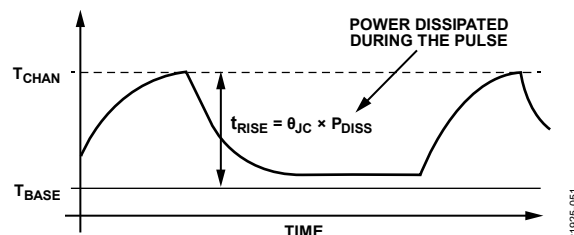
Figure 52. Pulsed Bias at Low Duty Cycle
