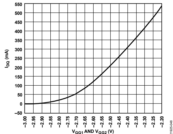
Figure 48. I_{DQ} vs. V_{GG1} and V_{GG2} , V_{DD1} and V_{DD2} = 50\text{ V} , Representative of a Typical Device
