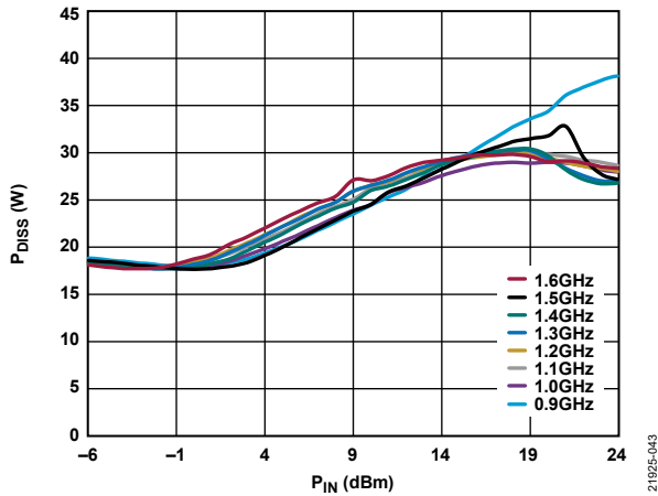
Figure 43. P_{DISS} vs. P_{IN} , Drain Bias Pulse Width = 100 \mu s at 10% Duty Cycle, T_{BASE} = 85^{\circ}\text{C}
