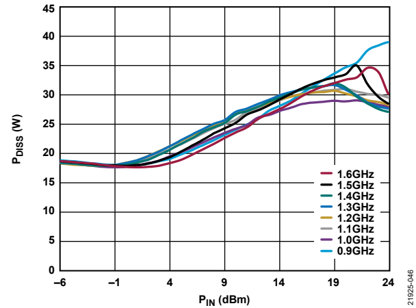
Figure 46. P_{DISS} vs. P_{IN} , Drain Bias Pulse Width = 200 \mu s at 20% Duty Cycle, T_{BASE} = 85^{\circ}\text{C}
