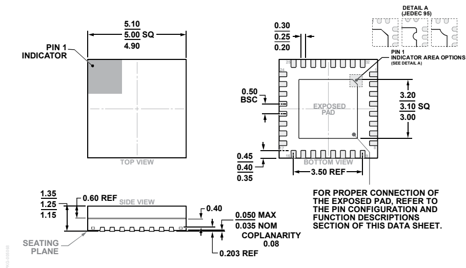
Figure 53. 32-Lead Lead frame Chip Scale Package, Premolded Cavity [LFCSP_CAV] 5 mm x 5 mm Body and 1.25 mm Package Height (CG-32-2) Dimensions shown in millimeters
