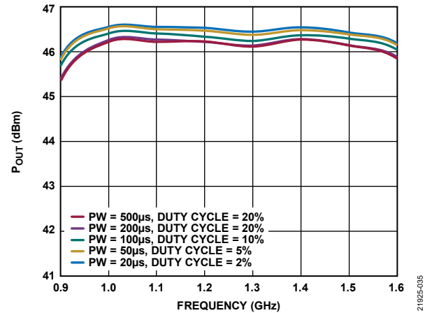
Figure 35. P_{OUT} vs. Frequency at Various Pulse Widths and Duty Cycles, P_{IN} = 19 dBm
