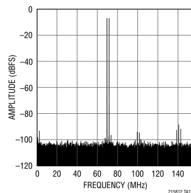
LTC2158-12 32K Point 2-Tone FFT, f_{\text{IN}} = 71\text{MHz} and 69\text{MHz} , 310Mps
