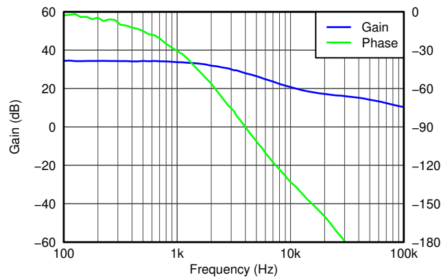
Figure 8-2. Power Stage Gain and Phase of the Boost Converter
