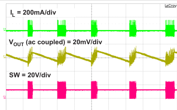
Figure 8-7. Pulse Skipping
