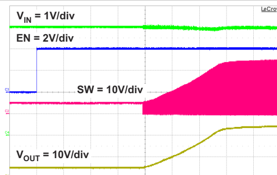
Figure 8-8. Start-Up
