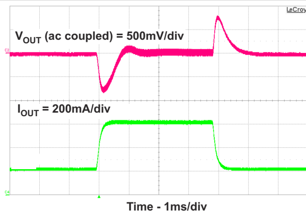
Figure 8-4. Load Transient Response
