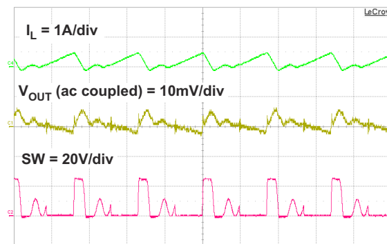
Figure 8-6. DCM PWM Operation
