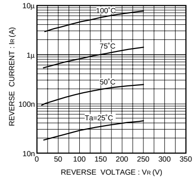
Fig.2 Reverse characteristics
