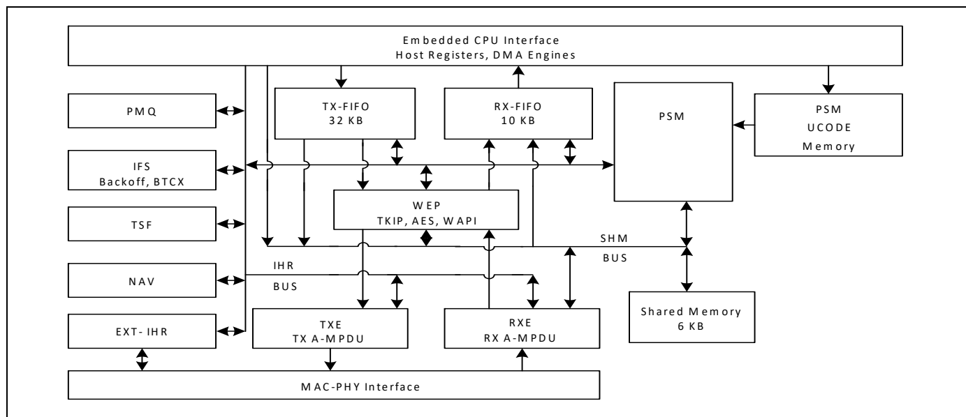
Figure 26. WLAN MAC Architecture
