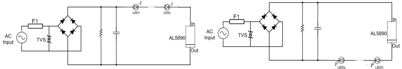
(AC Configuration)
