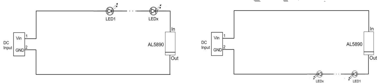
(DC Configuration)
