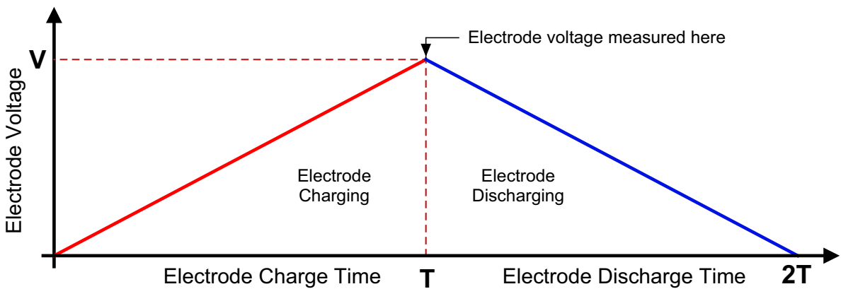
Figure 21. MPR03X Electrode Measurement Charging Pad Capacitance
