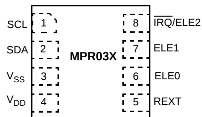
Figure 1. Pin Connections
