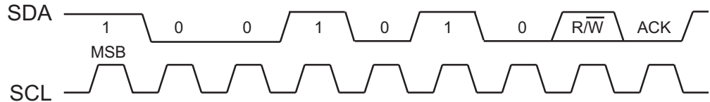
Figure 9. Slave Address
