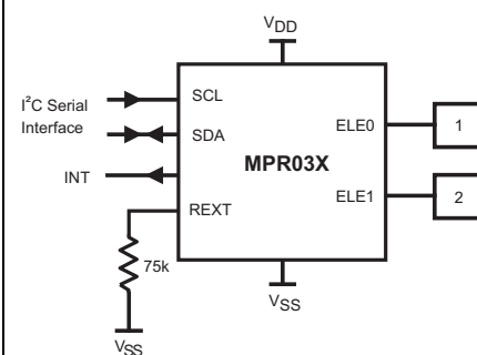
MPR03X with 2 Electrodes and 2 Pads
