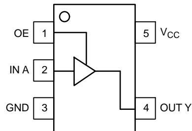
Figure 2. SC-88A (Top View)
