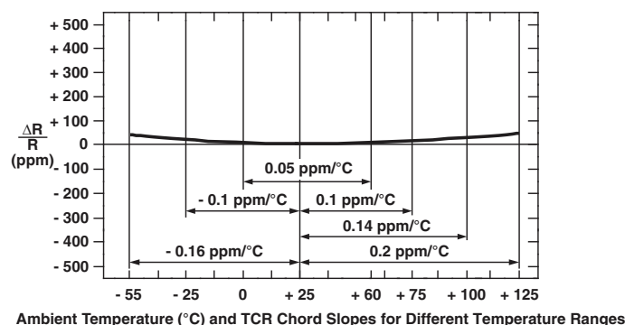
FIGURE 4 - TYPICAL RESISTANCE/TEMPERATURE CURVE
