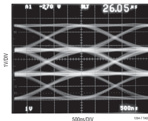
4-Level PAM Eye Diagram
