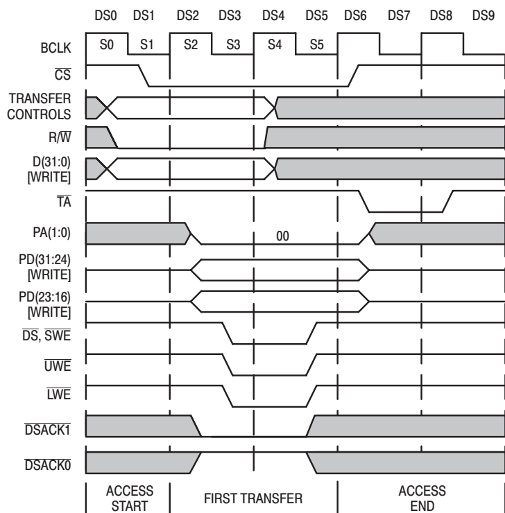
Figure 26. 16-Bit '040 WRITE to 16-Bit Peripheral Example (PA1=0)
