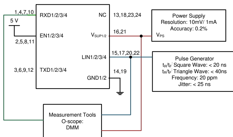
Figure 8-1. Test System: Operating Voltage Range with RX and TX Access
