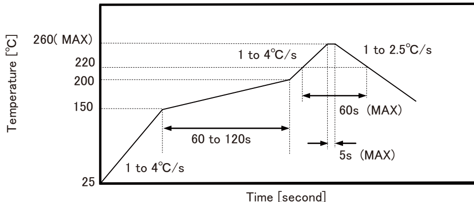
Temperature Profile
