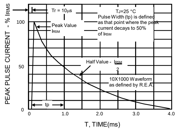
FIG.2 - PULSE WAVEFORM
