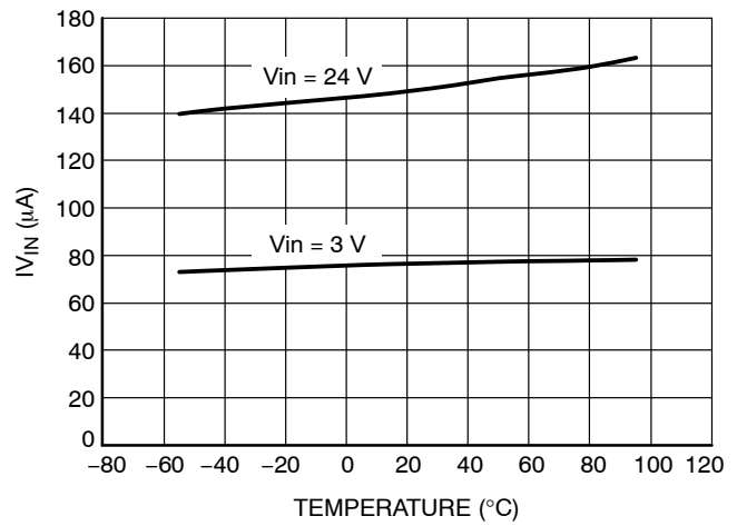
Figure 12. V_{in} Controller Current vs. Temperature ( \text{EN} = \text{HIGH} )
