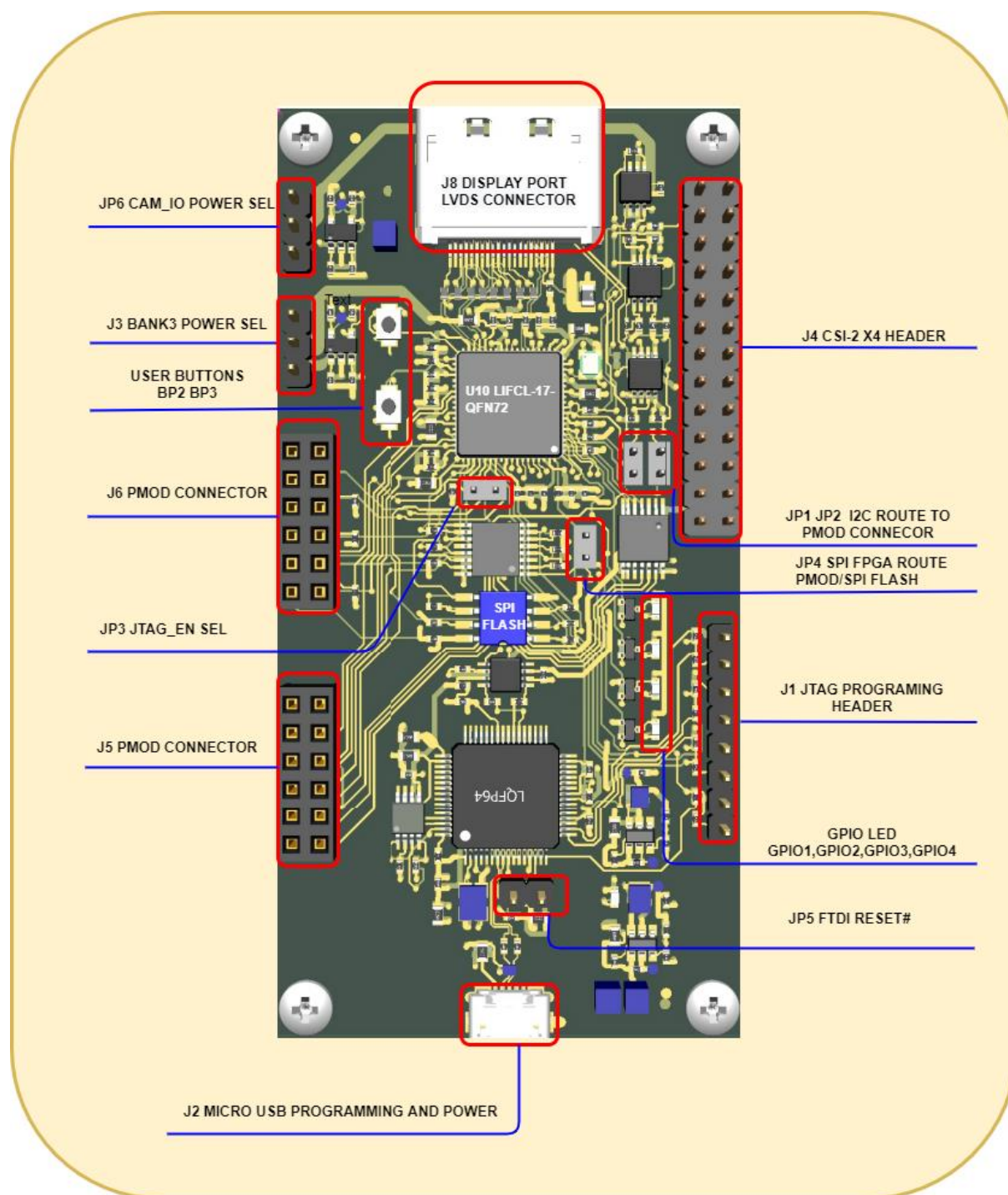
FIGURE 2 TOP OF THE BOARD
