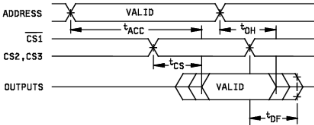
FIGURE 5. AC read timing diagram.
