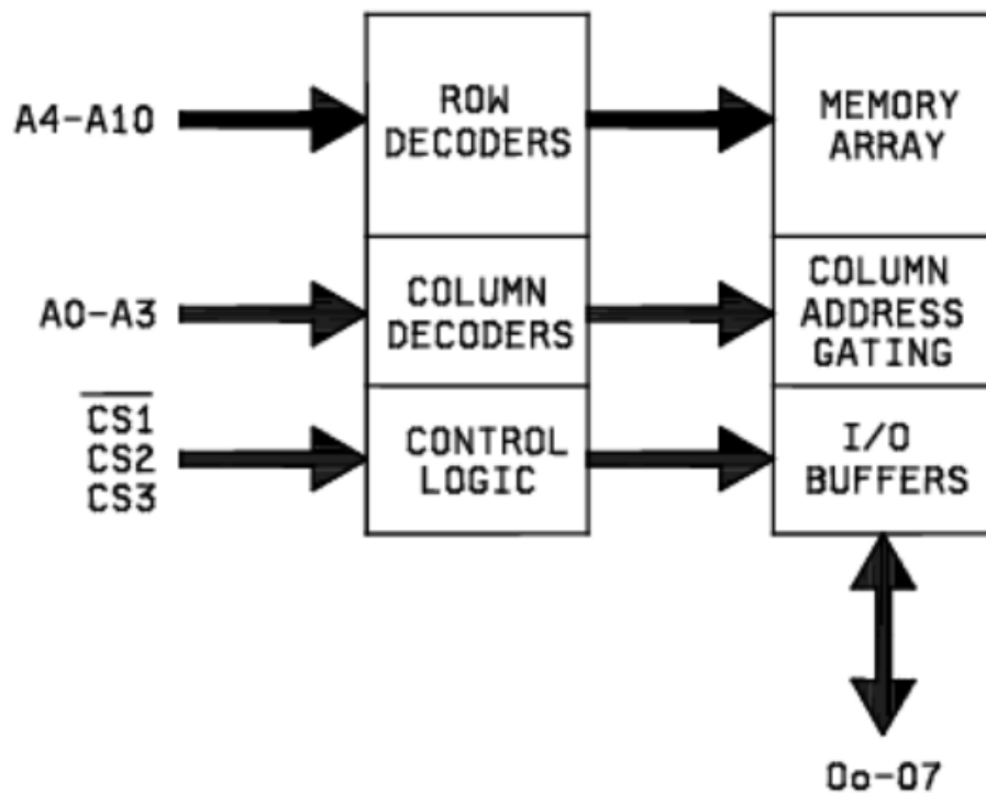
FIGURE 3. Block diagram.
