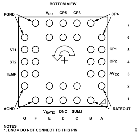
Figure 3. Pin Configuration
