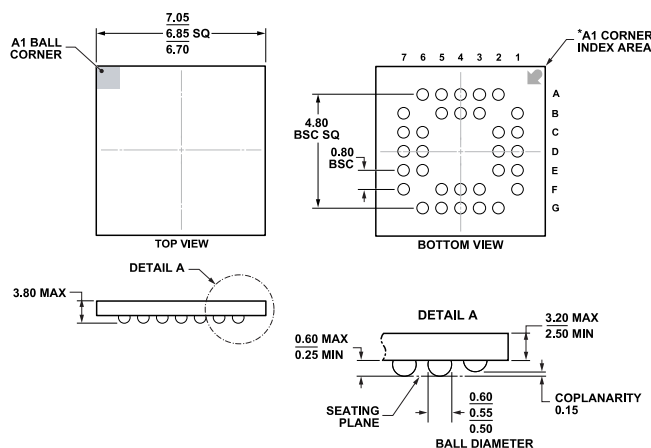
Figure 19. 32-Lead Ceramic Ball Grid Array [CBGA] (BG-32-3) Dimensions shown in millimeters
