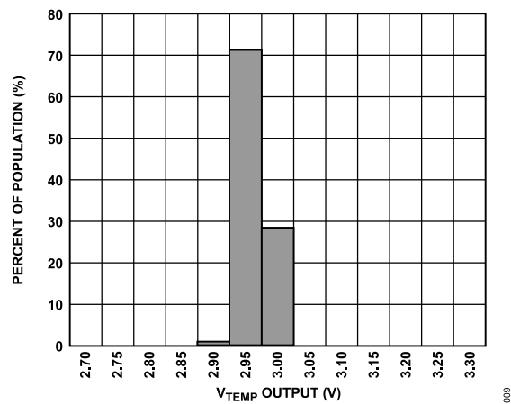
Figure 16. V_{TEMP} Output at 25°C ( V_{RATIO} = 5\text{ V} )
