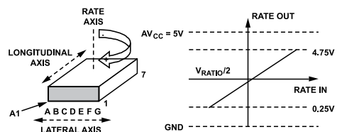
Figure 2. RATEOUT Signal Increases with Clockwise Rotation
