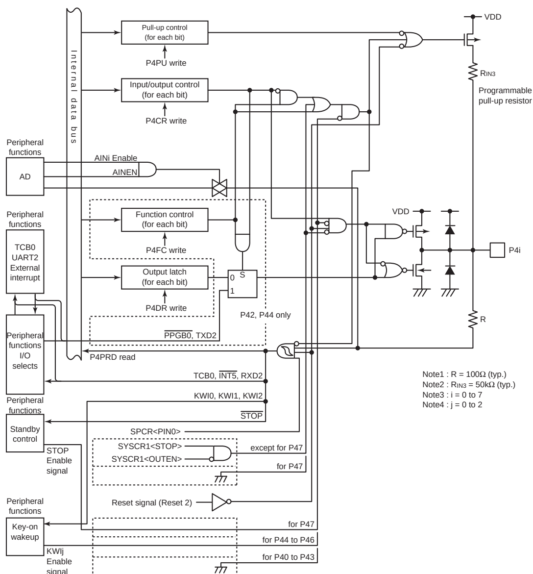
Figure 8-7 Port P4
