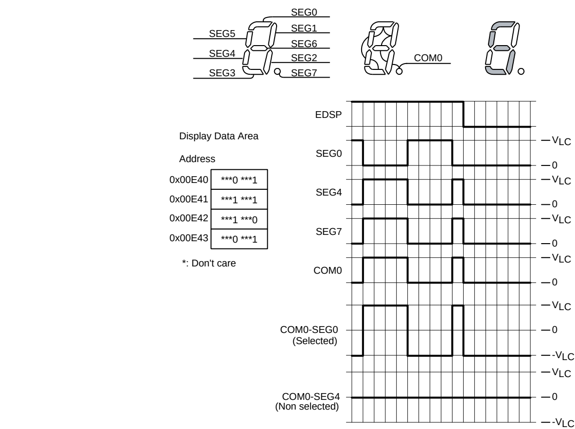
Figure 23-12 Static Drive
