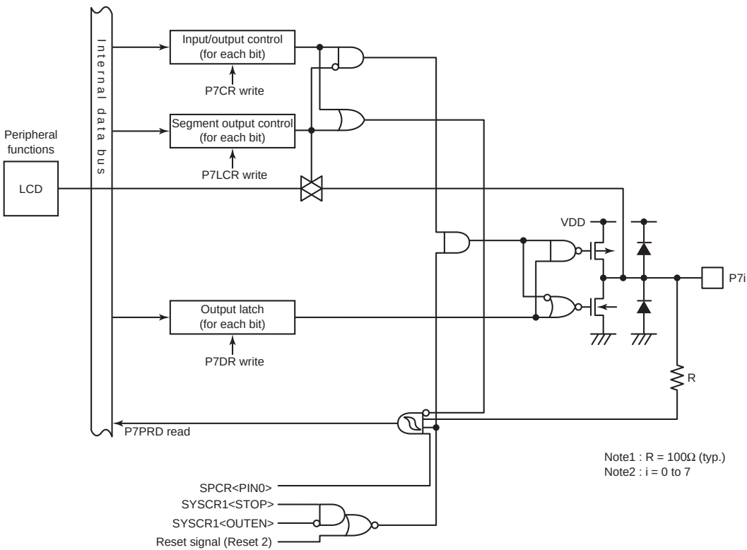
Figure 8-10 Port P7
