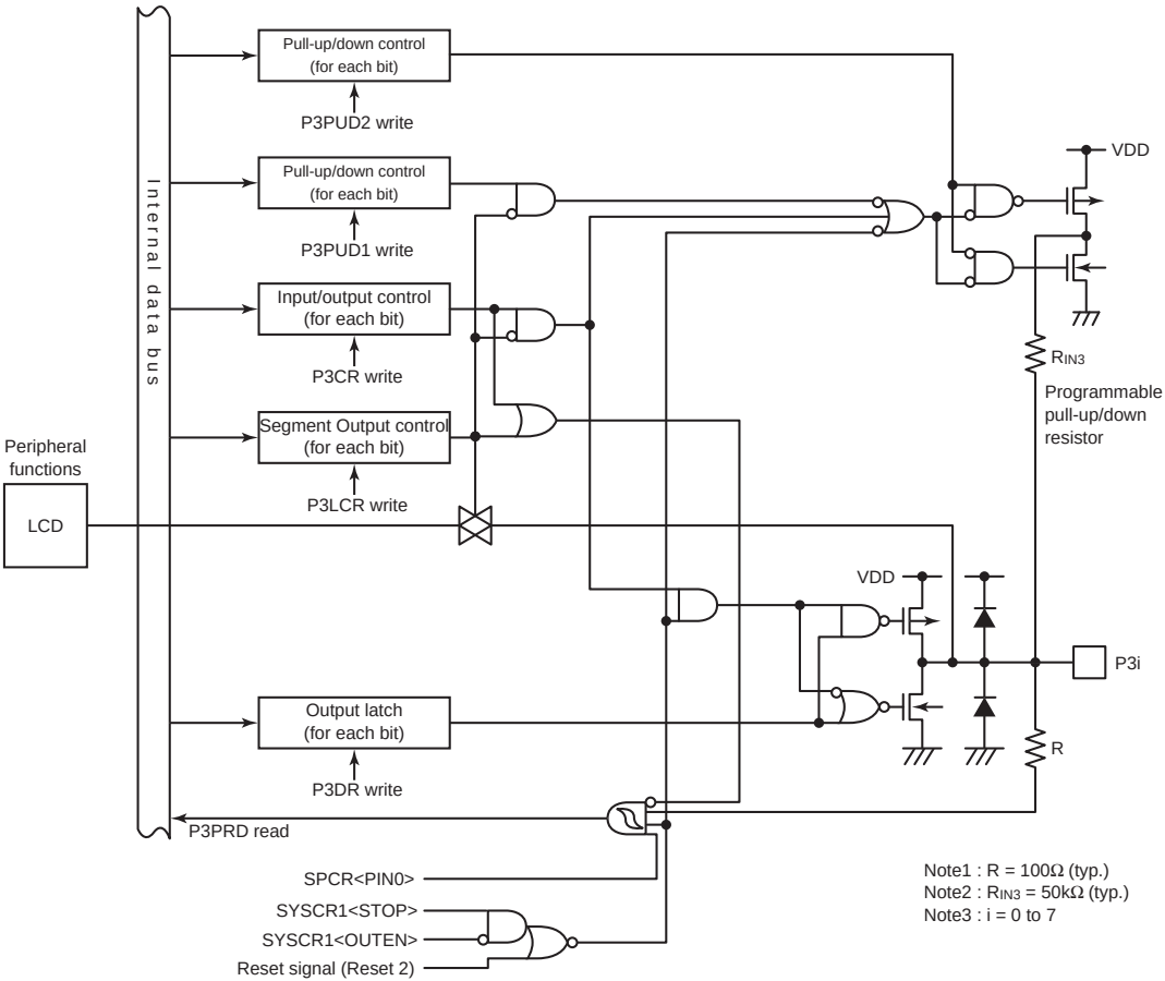
Figure 8-6 Port P3
