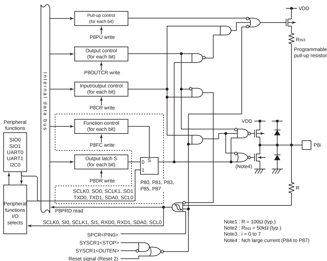
Figure 8-11 Port P8
