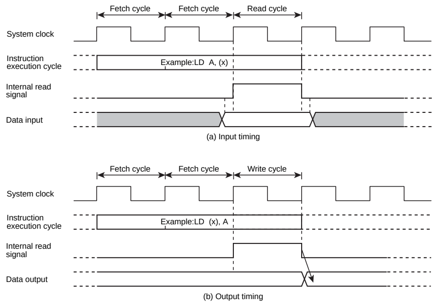
Figure 8-1 Input/Output Timing(Example)
