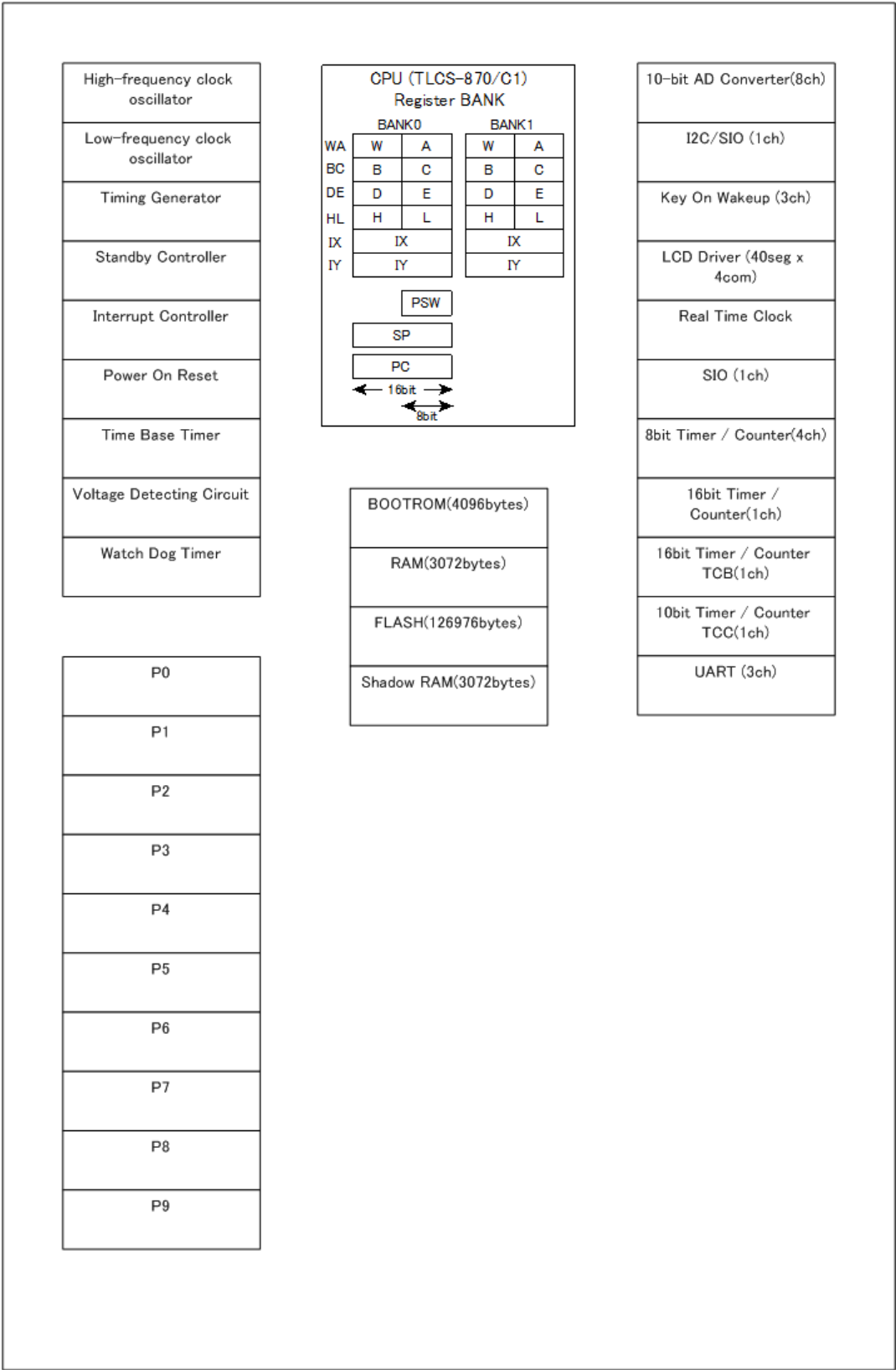
Figure 1-2 Block Diagram
