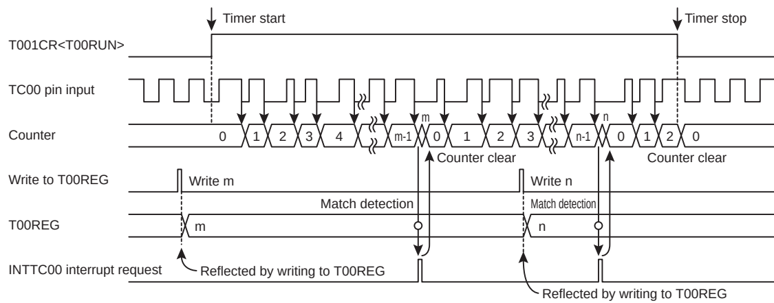
Figure 16-4 Event Counter Mode Timing Chart
