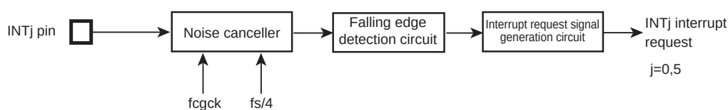
Figure 4-1 External Interrupts 0/5
