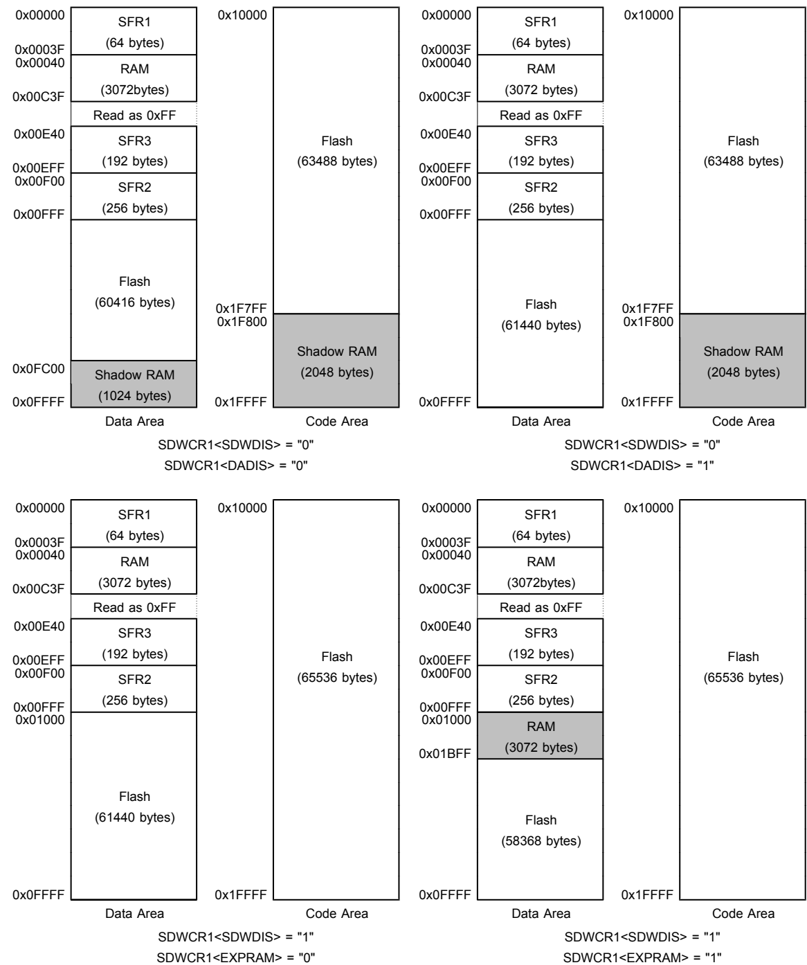
Figure 25-2 Memory Map
