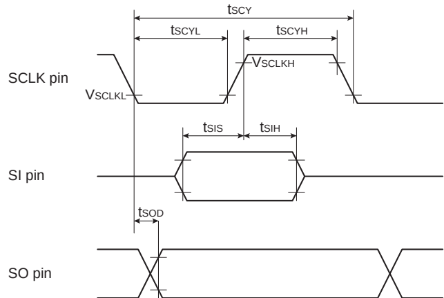
Figure 19-17 AC Characteristics
