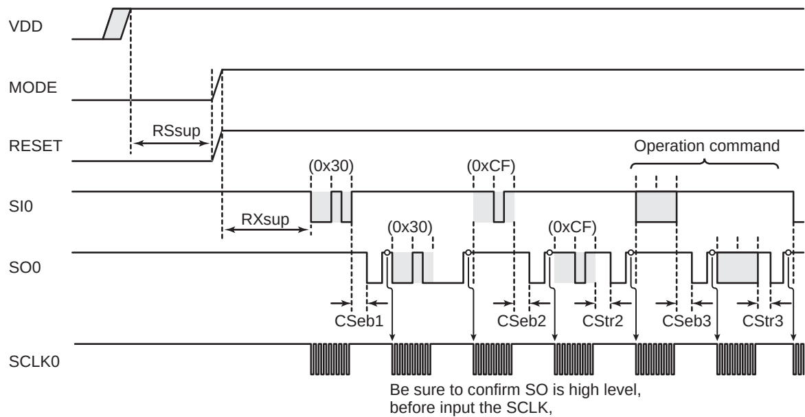
Figure 26-17 Reset Timing
