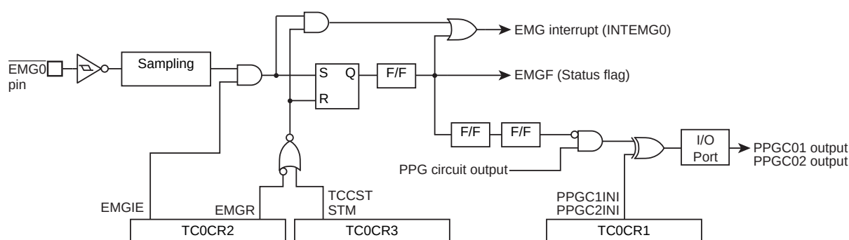
Figure 15-22 \overline{\text{EMG0}} Pin
