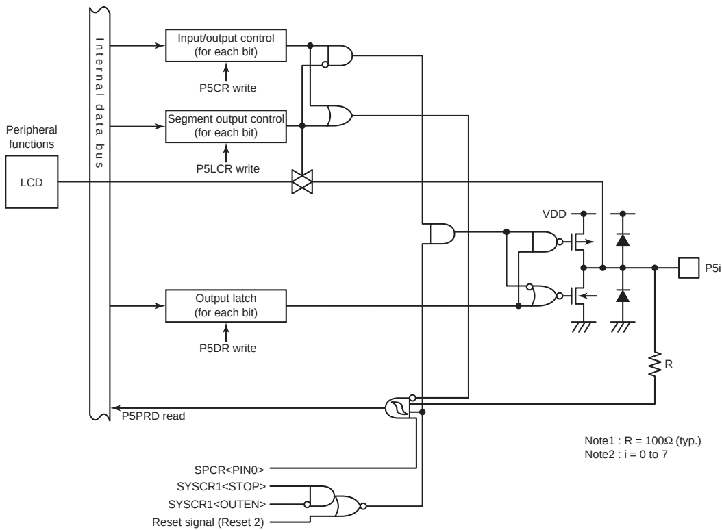
Figure 8-8 Port P5
