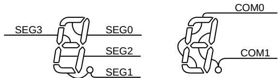
Figure 23-7 Example of COM and SEG Pin Connections
