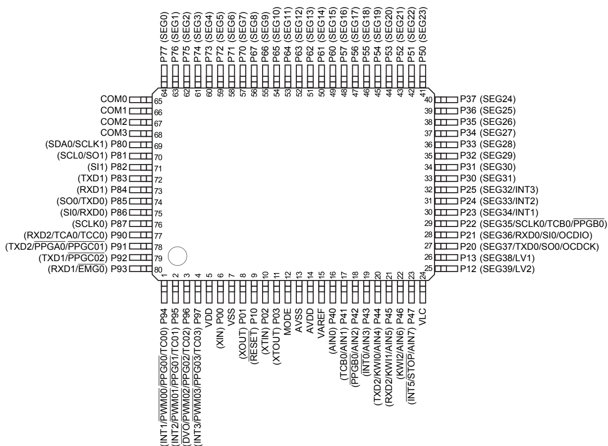
TMP89FW24ADFG (QFP80-P-1420-0.80M)
