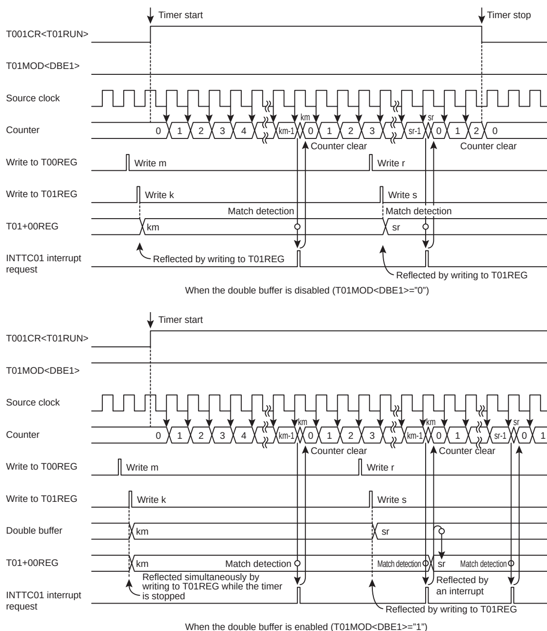
Figure 16-11 16-bit Timer Counter Timing Chart
