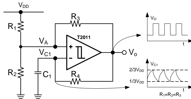
Figure 8. Relaxation Oscillator
