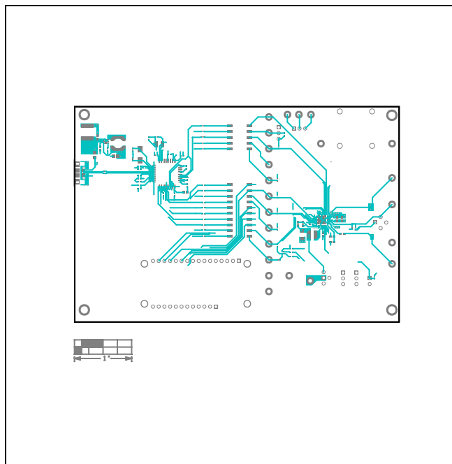
MAX22516 EV Kit PCB Layout—Layer 2
