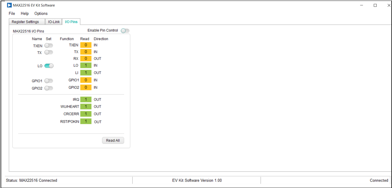
Figure 3. I/O Pin Tab in the MAX22516 EV Kit GUI
