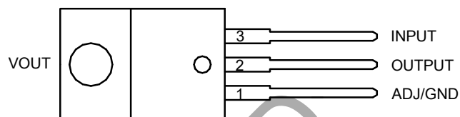
TO220-3 (Option 2)
