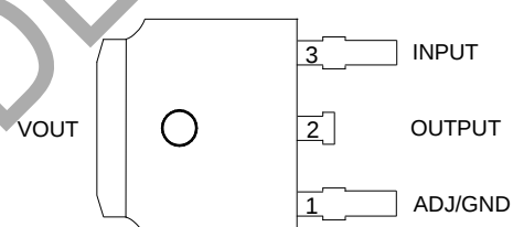
TO252-2 (3) (Option 2) / TO252 (Type CJ)
