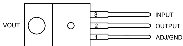
TO220-3 (Option 3)
