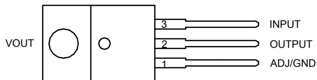
TO220-3 (Option 1)
