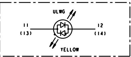
BI-COLOR LED
