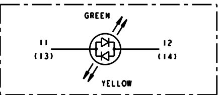
BI-COLOR LED
