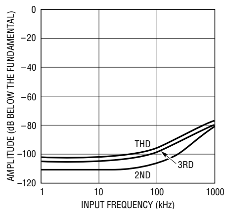
Figure 5. Distortion vs Input Frequency
