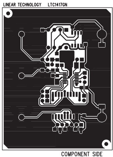
Figure 13c. Suggested Evaluation Circuit Board—Component Side
