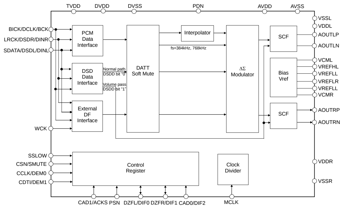
Block Diagram
