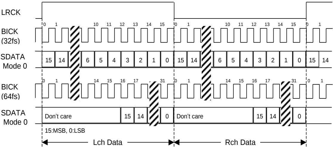
Figure 11. Mode 0 Timing
