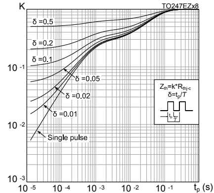
Figure 2. Thermal impedance
